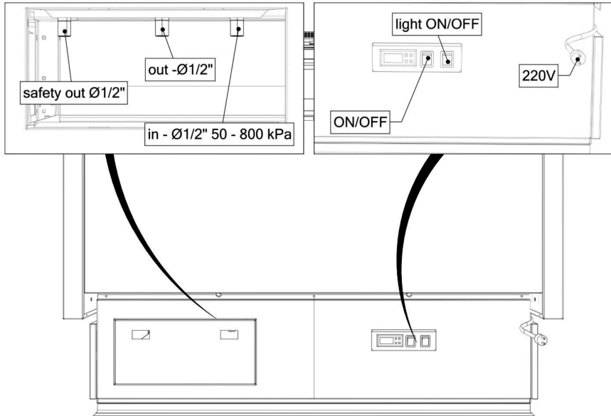
Fig.1. Connection diagram for water and electricity installations
